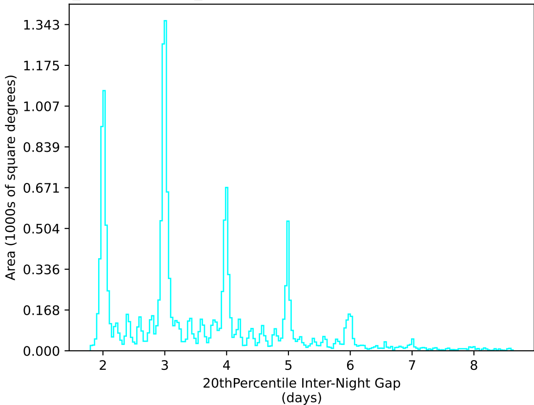
weather_cloudso20v3.4_10yrs WFD u band: 20thPercentile Inter-Night Gap
