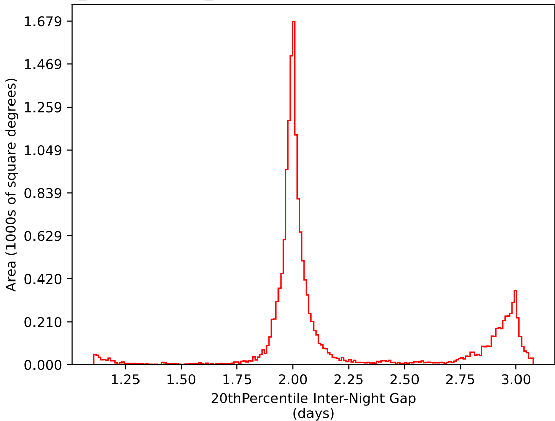
weather_cloudso20v3.4_10yrs WFD i band: 20thPercentile Inter-Night Gap
