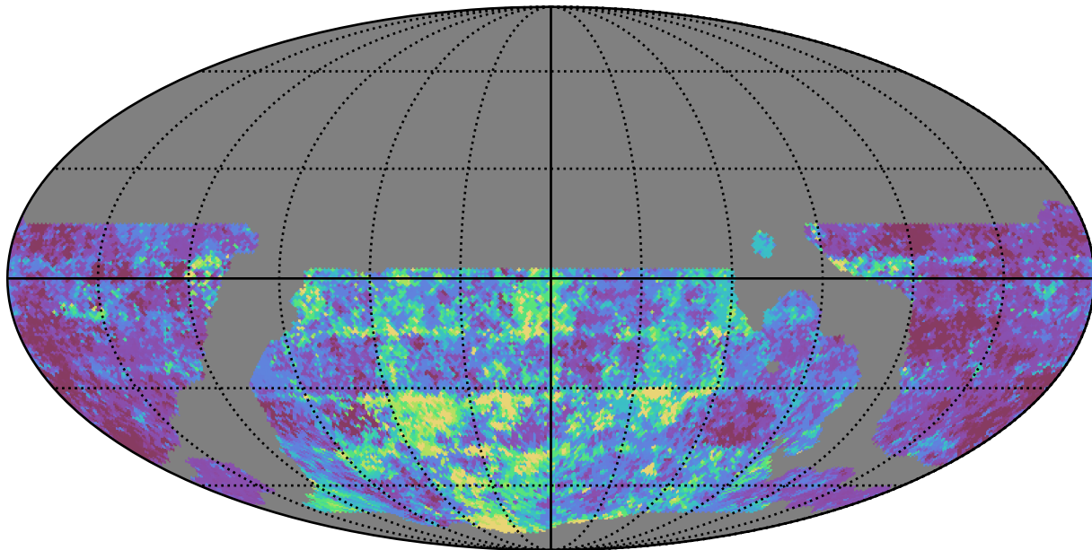
weather_cloudso20v3.4_10yrs WFD g band: 20thPercentile Inter-Night Gap
