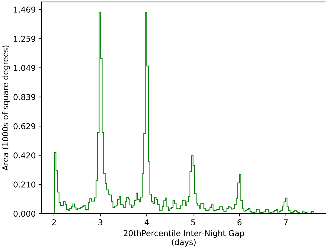
weather_cloudso20v3.4_10yrs WFD g band: 20thPercentile Inter-Night Gap
