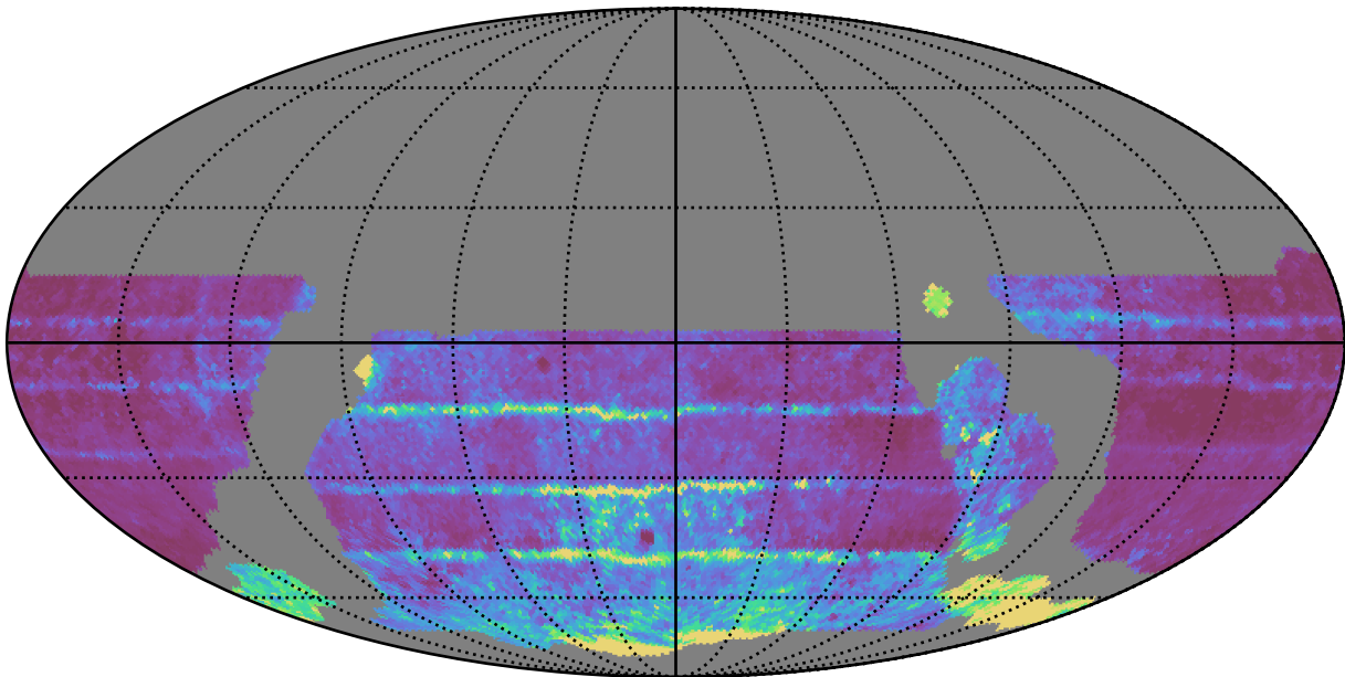
weather_cloudso20v3.4_10yrs WFD all bands: 20thPercentile Inter-Night Gap
