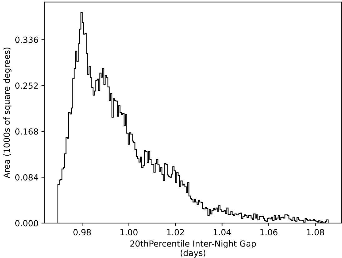
weather_cloudso20v3.4_10yrs WFD all bands: 20thPercentile Inter-Night Gap
