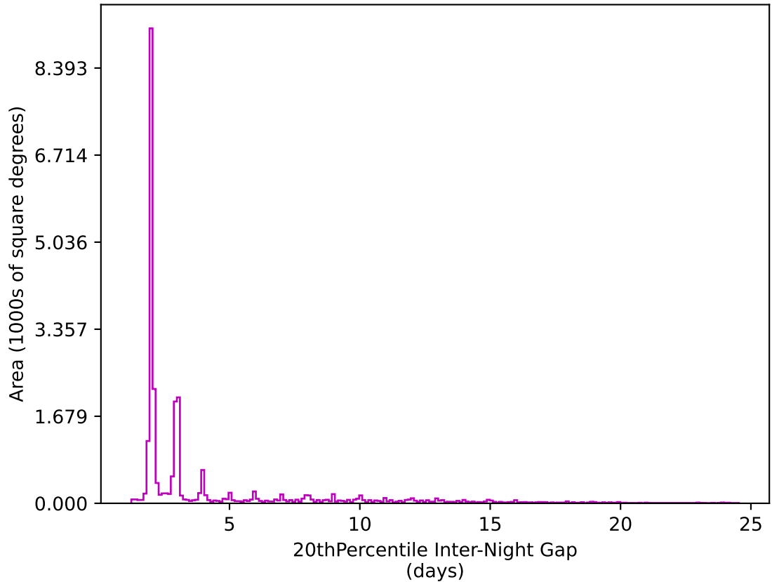
weather_cloudso20v3.4_10yrs All sky z band: 20thPercentile Inter-Night Gap
