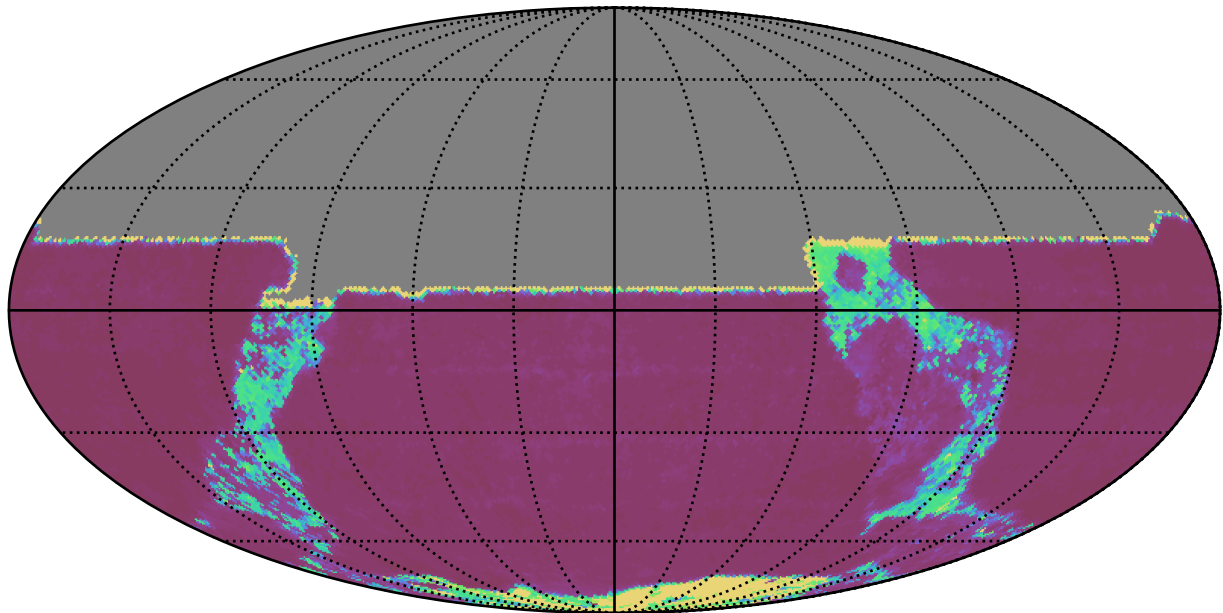
weather_cloudso20v3.4_10yrs All sky y band: 20thPercentile Inter-Night Gap
