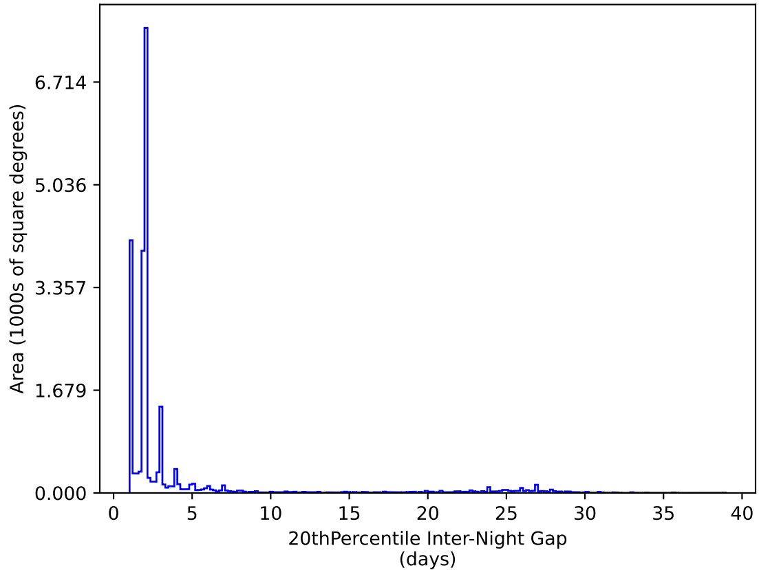
weather_cloudso20v3.4_10yrs All sky y band: 20thPercentile Inter-Night Gap
