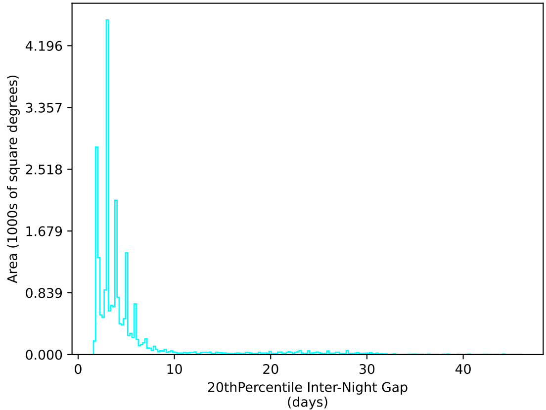
weather_cloudso20v3.4_10yrs All sky u band: 20thPercentile Inter-Night Gap
