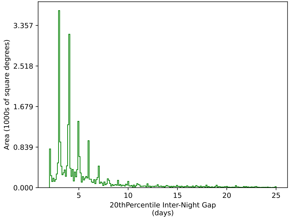
weather_cloudso20v3.4_10yrs All sky g band: 20thPercentile Inter-Night Gap
