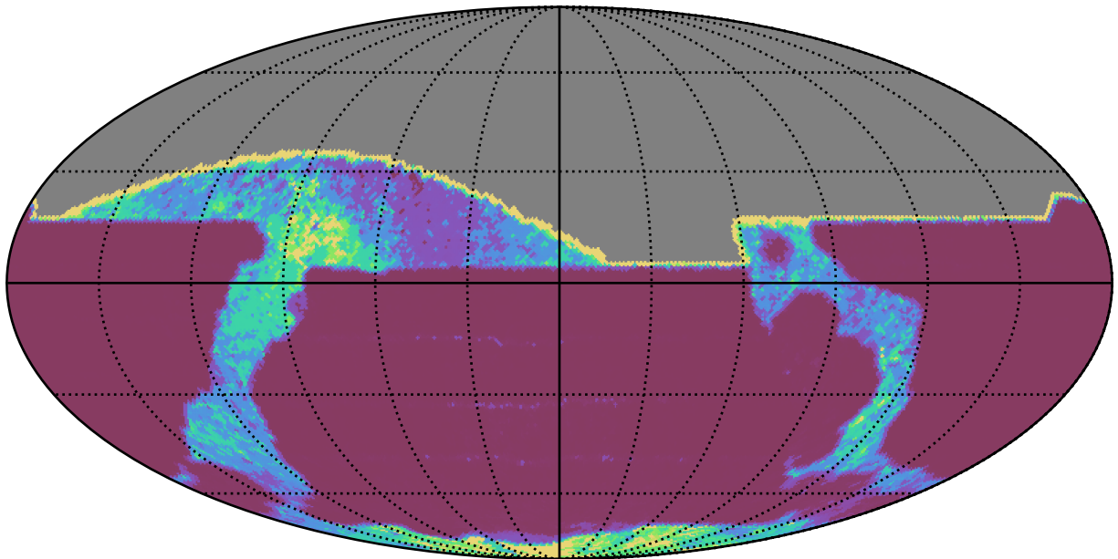
weather_cloudso20v3.4_10yrs All sky all bands: 20thPercentile Inter-Night Gap
