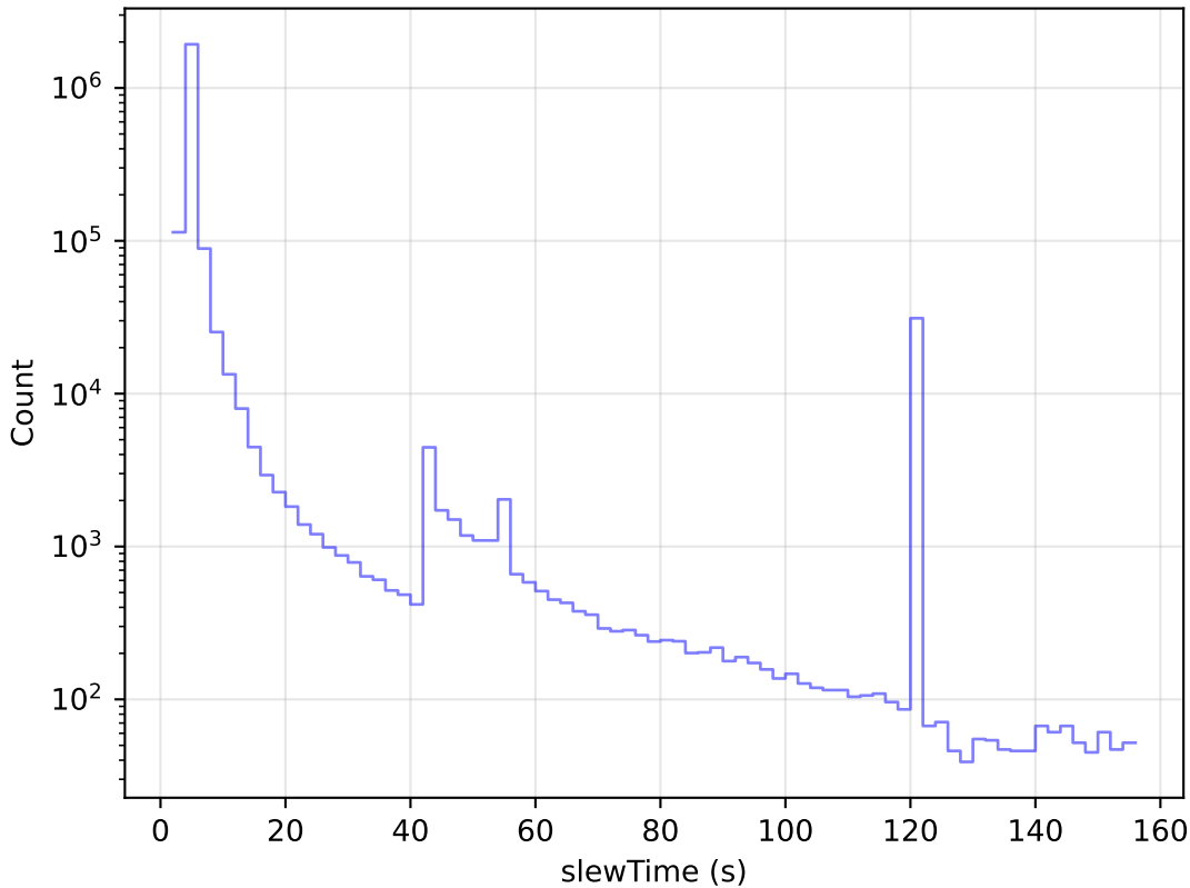
weather_cloudso20v3.4_10yrs All visits: Slew Time Histogram
