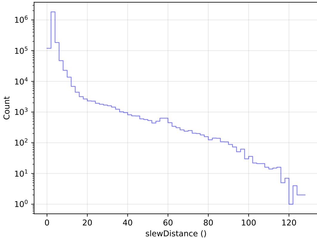
weather_cloudso20v3.4_10yrs All visits: Slew Distance Histogram
