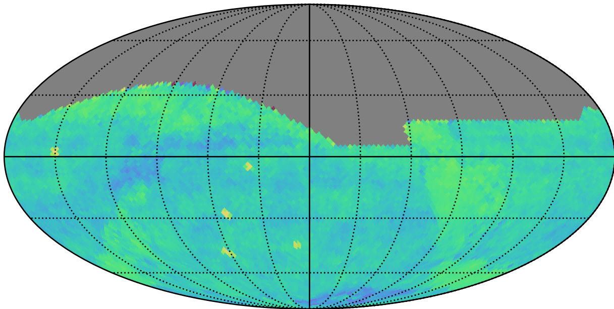
weather_cloudso20v3.4_10yrs (g or r or i): PairFraction
