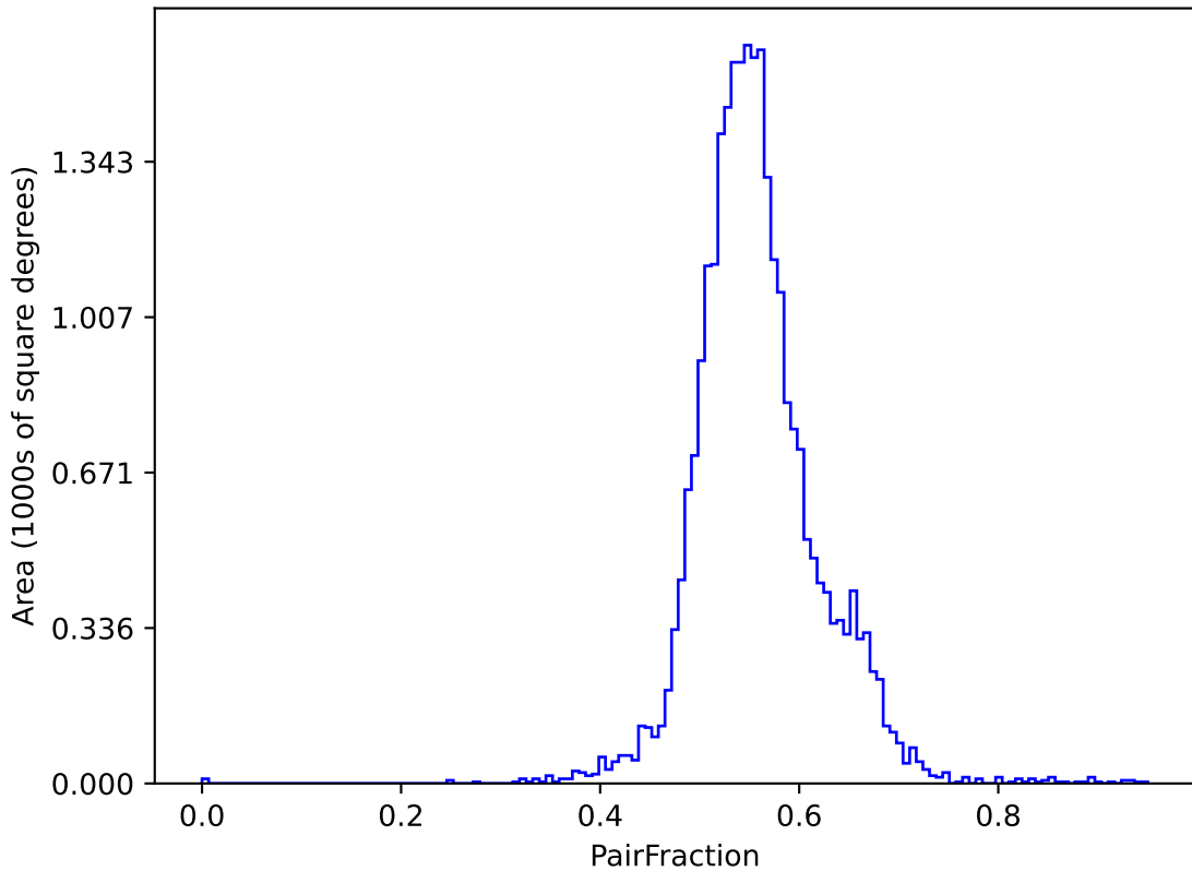
weather_cloudso20v3.4_10yrs (g or r or i): PairFraction
