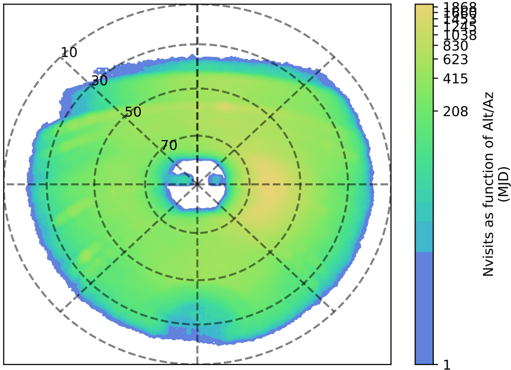
weather_cloudso20v3.4_10yrs y: Nvisits as function of Alt/Az
