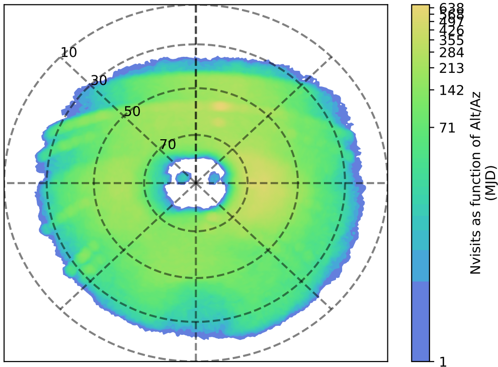
weather_cloudso20v3.4_10yrs u: Nvisits as function of Alt/Az
