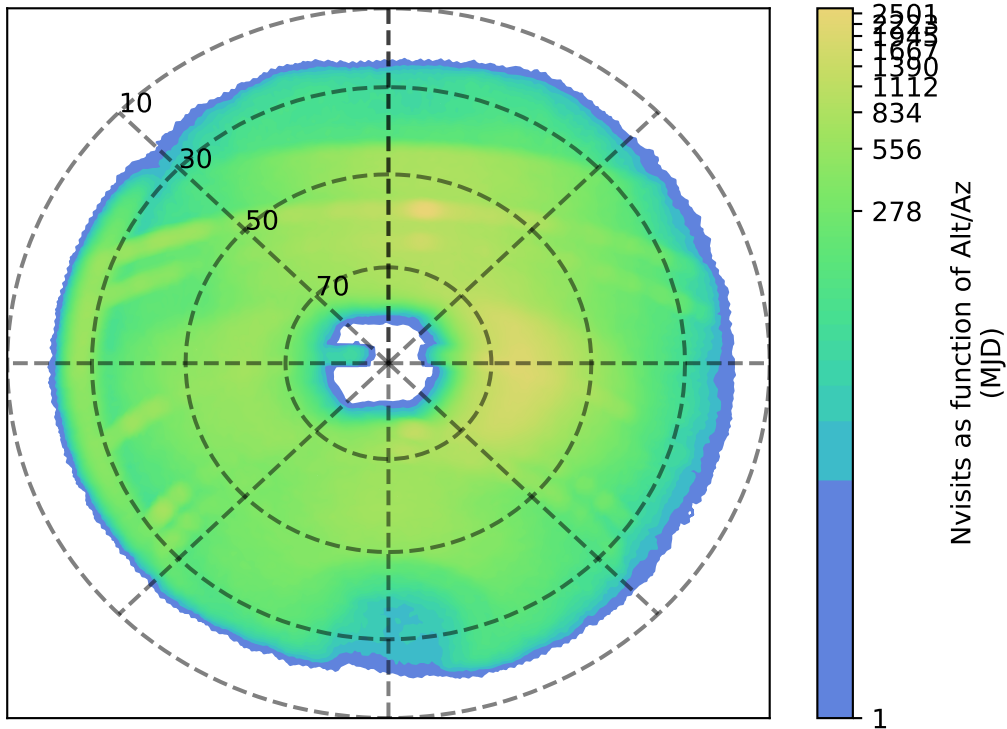
weather_cloudso20v3.4_10yrs r: Nvisits as function of Alt/Az
