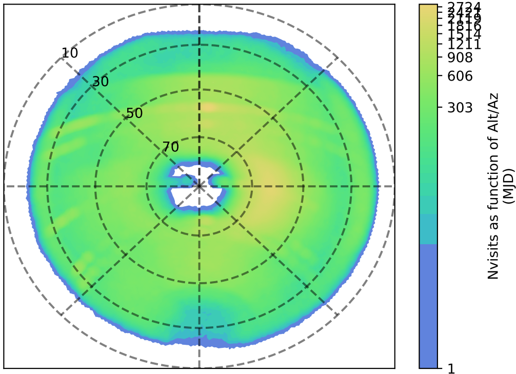
weather_cloudso20v3.4_10yrs i: Nvisits as function of Alt/Az
