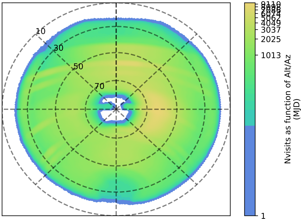
weather_cloudso20v3.4_10yrs : Nvisits as function of Alt/Az
