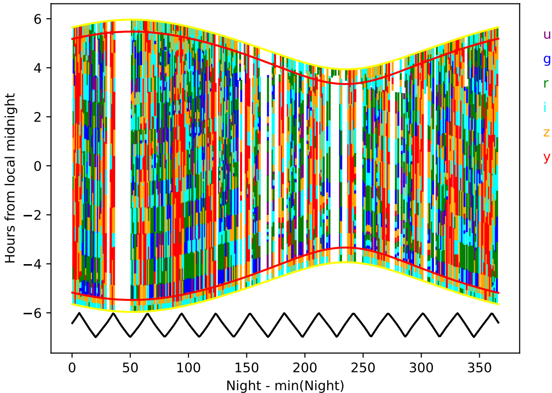
weather_cloudso20v3.4_10yrs year 6-7: Hourglass
