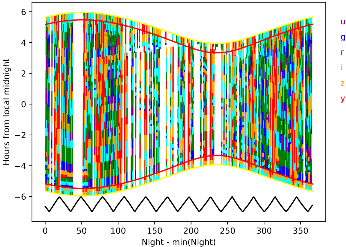
weather_cloudso20v3.4_10yrs year 2-3: Hourglass
