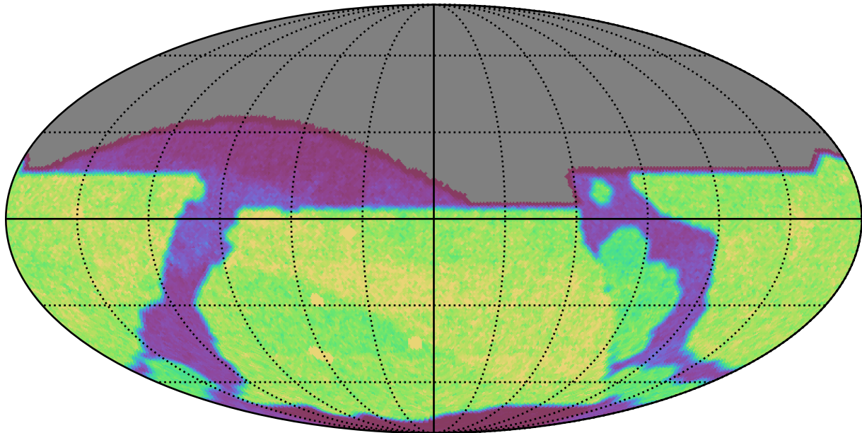
weather_cloudso20v3.4_10yrs z: Count observationStartMJD
