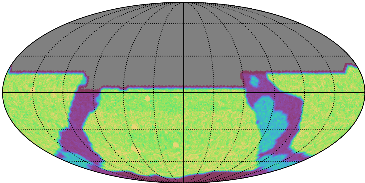
weather_cloudso20v3.4_10yrs y: Count observationStartMJD
