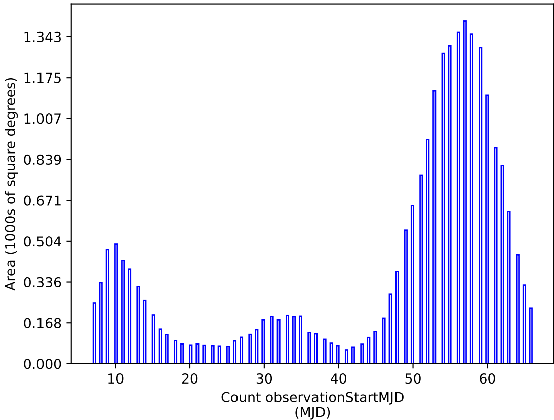
weather_cloudso20v3.4_10yrs u: Count observationStartMJD
