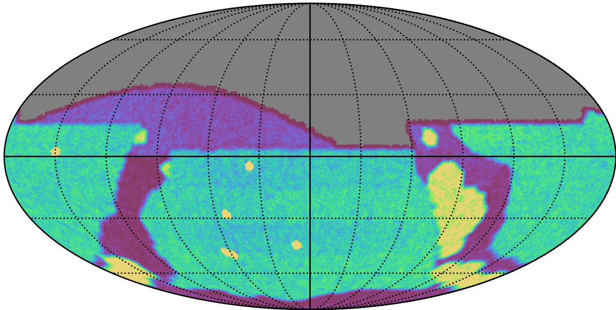
weather_cloudso20v3.4_10yrs g: Count observationStartMJD
