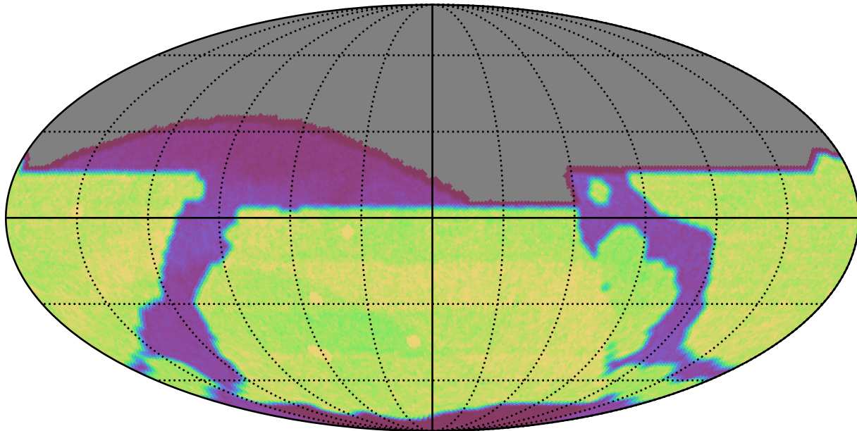
weather_cloudso20v3.4_10yrs : Count observationStartMJD
