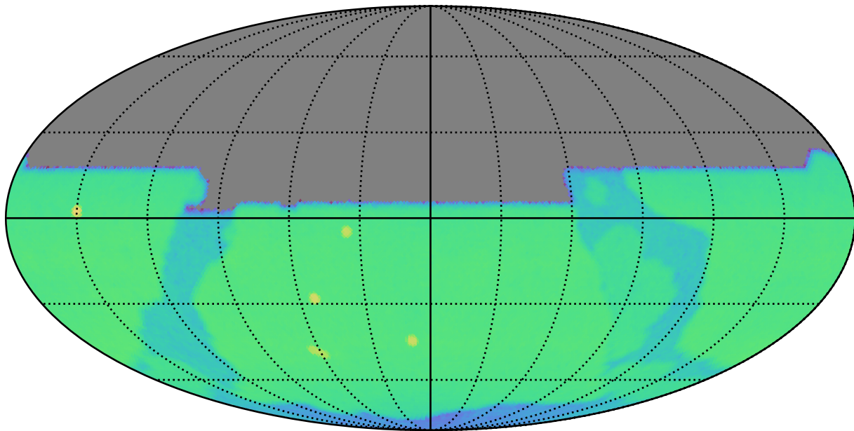
weather_cloudso20v3.4_10yrs y: CoaddM5
