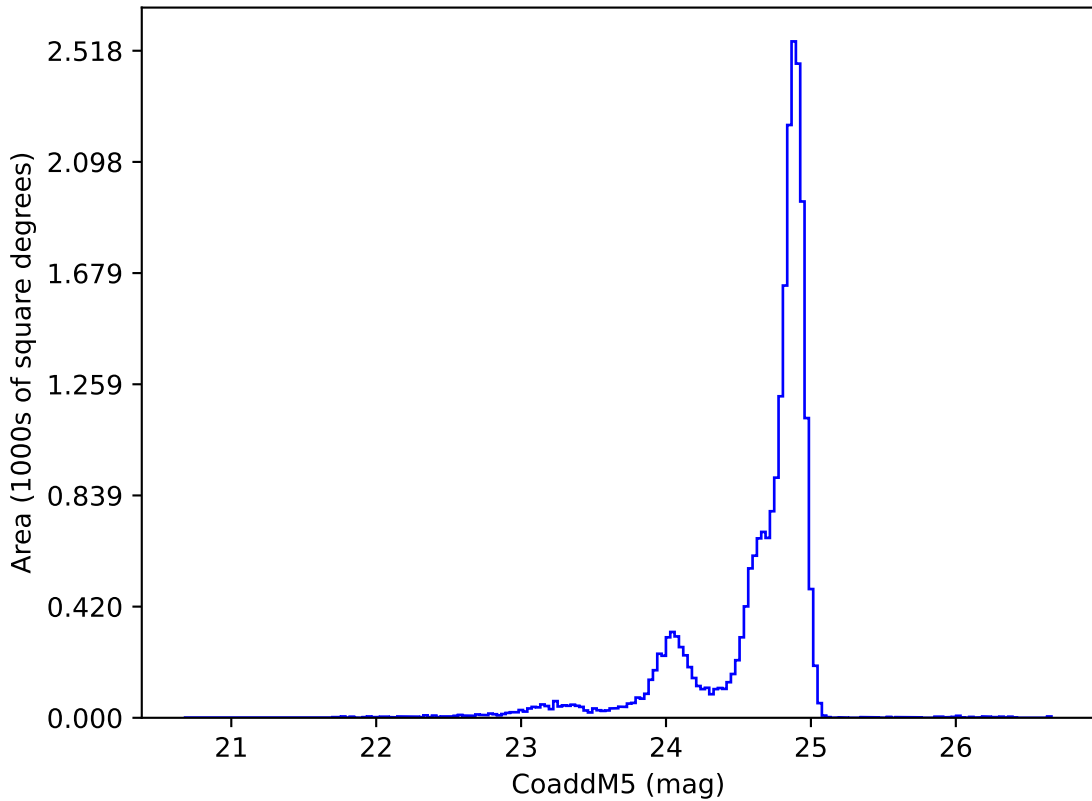
weather_cloudso20v3.4_10yrs y: CoaddM5
