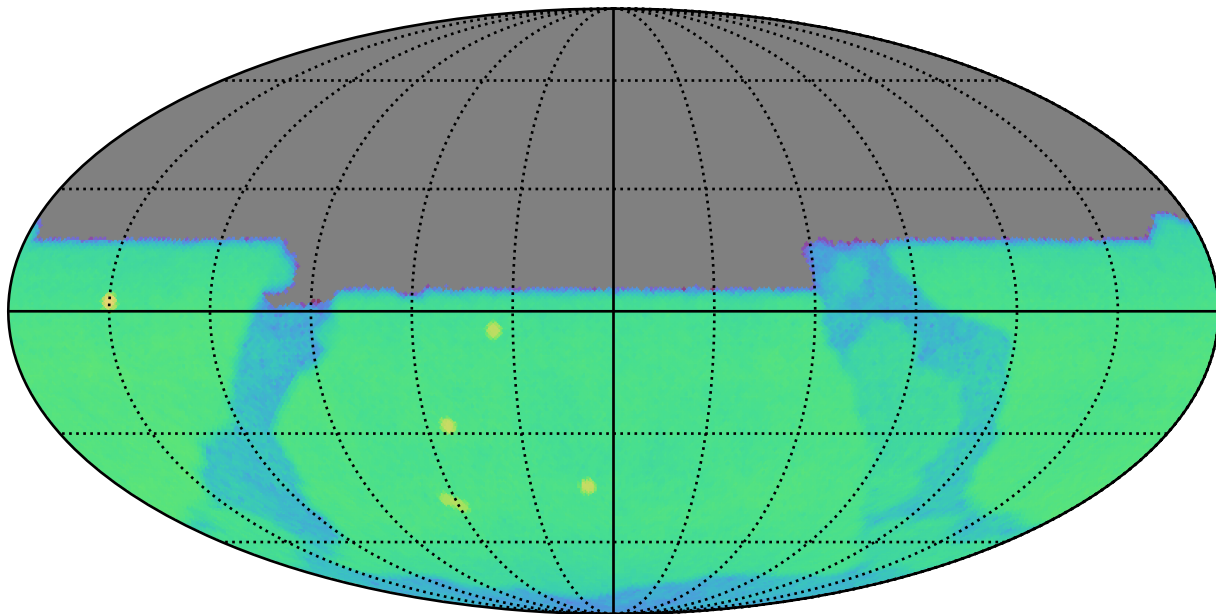
weather_cloudso20v3.4_10yrs u: CoaddM5
