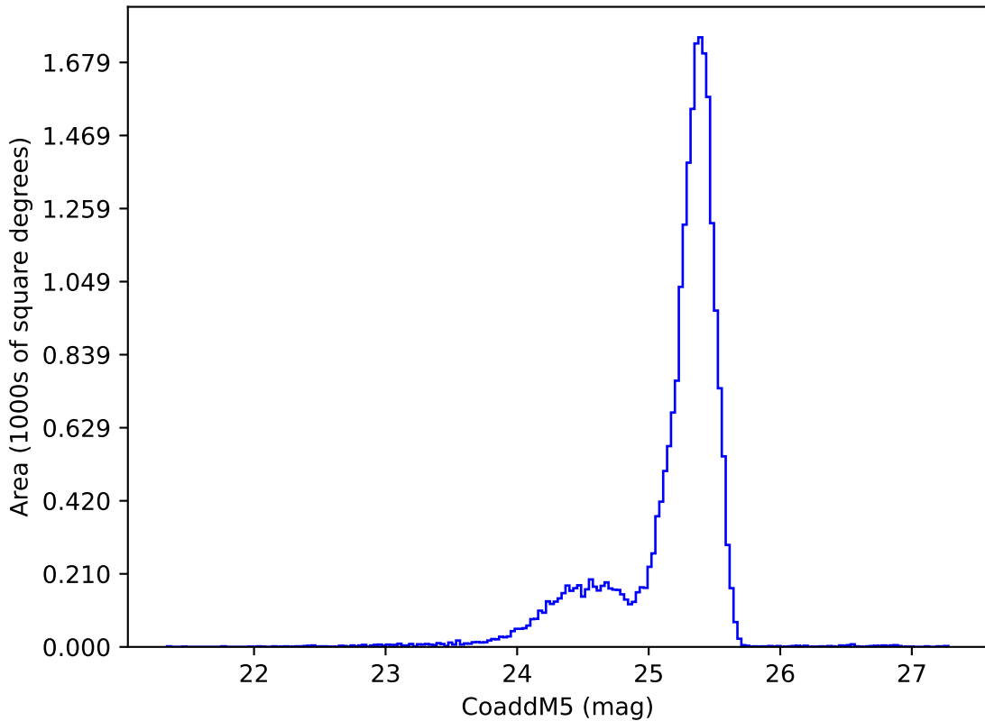
weather_cloudso20v3.4_10yrs u: CoaddM5
