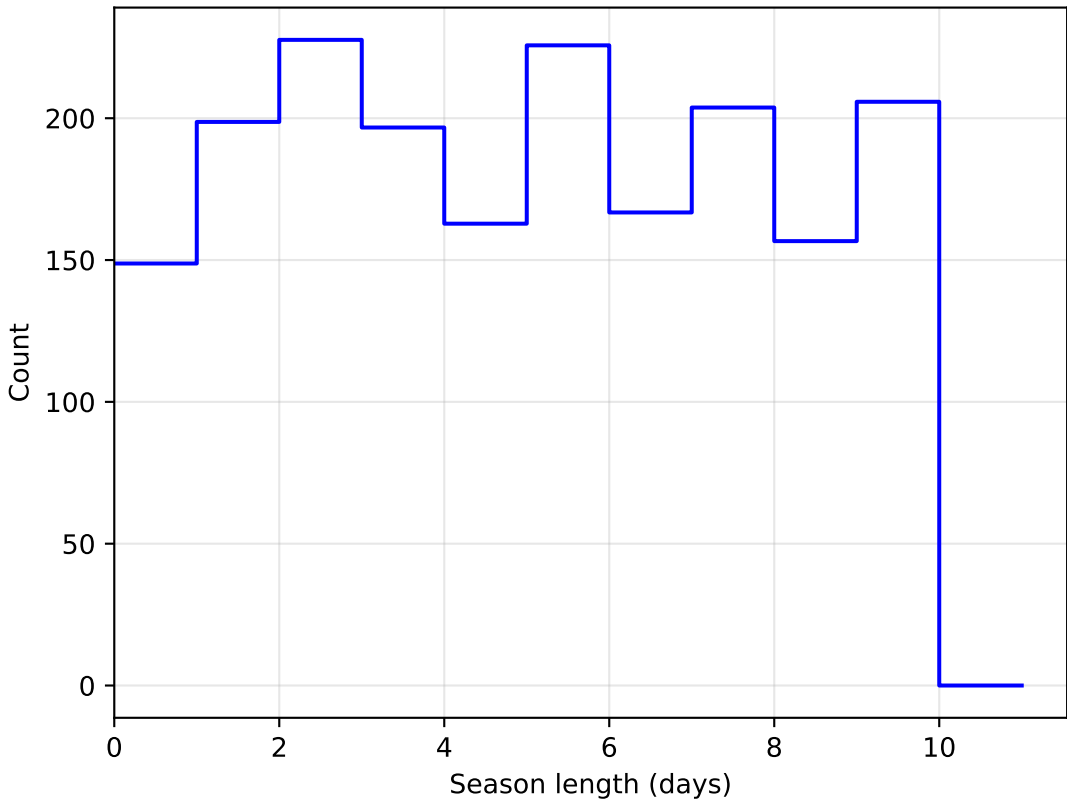
weather_cloudso20v3.4_10yrs DD:WFD all bands: SeasonLength
