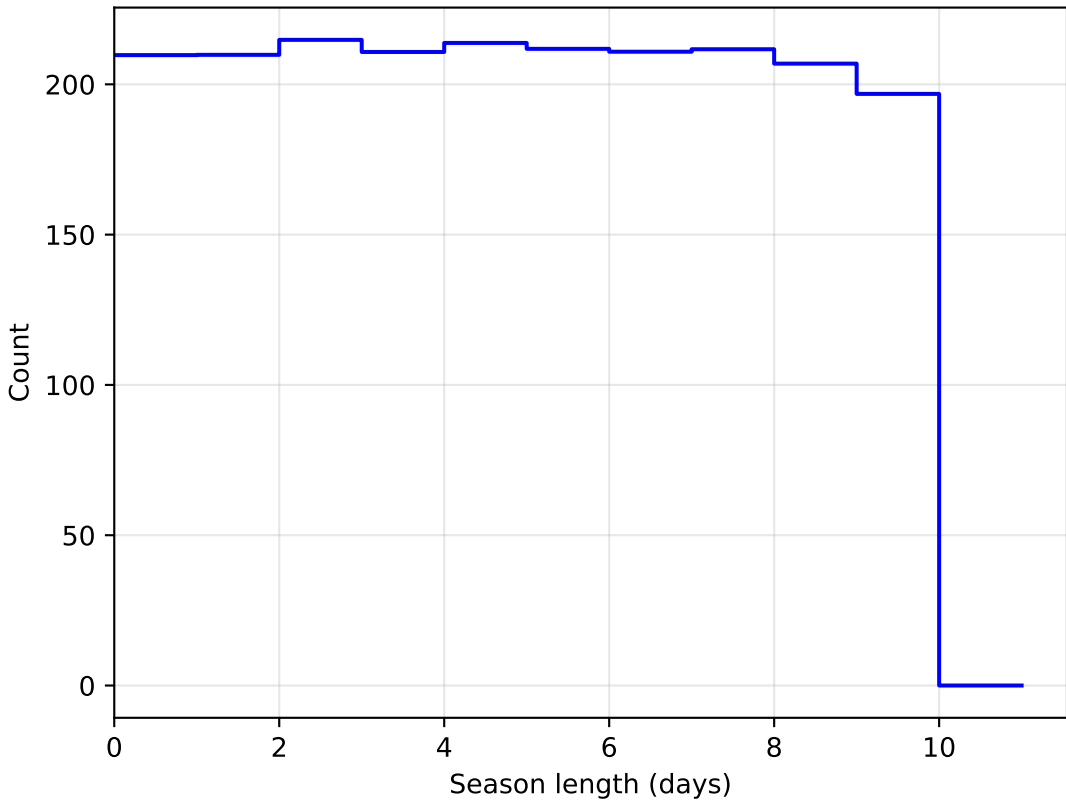
weather_cloudso20v3.4_10yrs DD:EDFS all bands: SeasonLength
