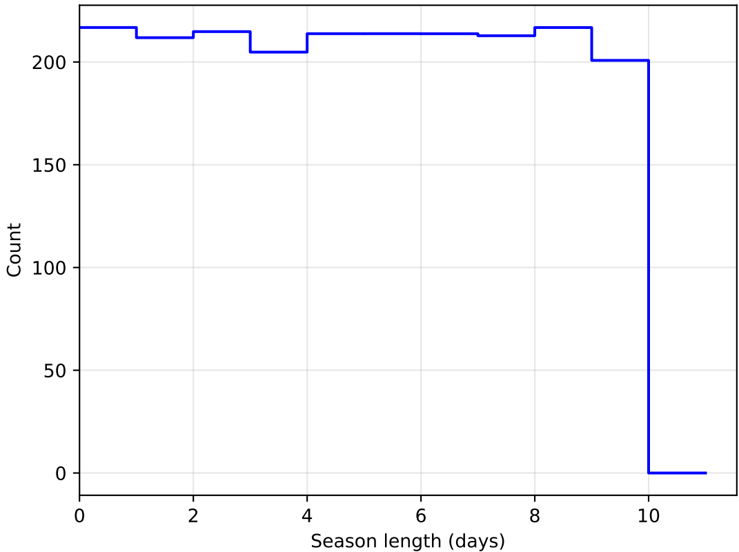
weather_cloudso20v3.4_10yrs DD:ECDFS all bands: SeasonLength
