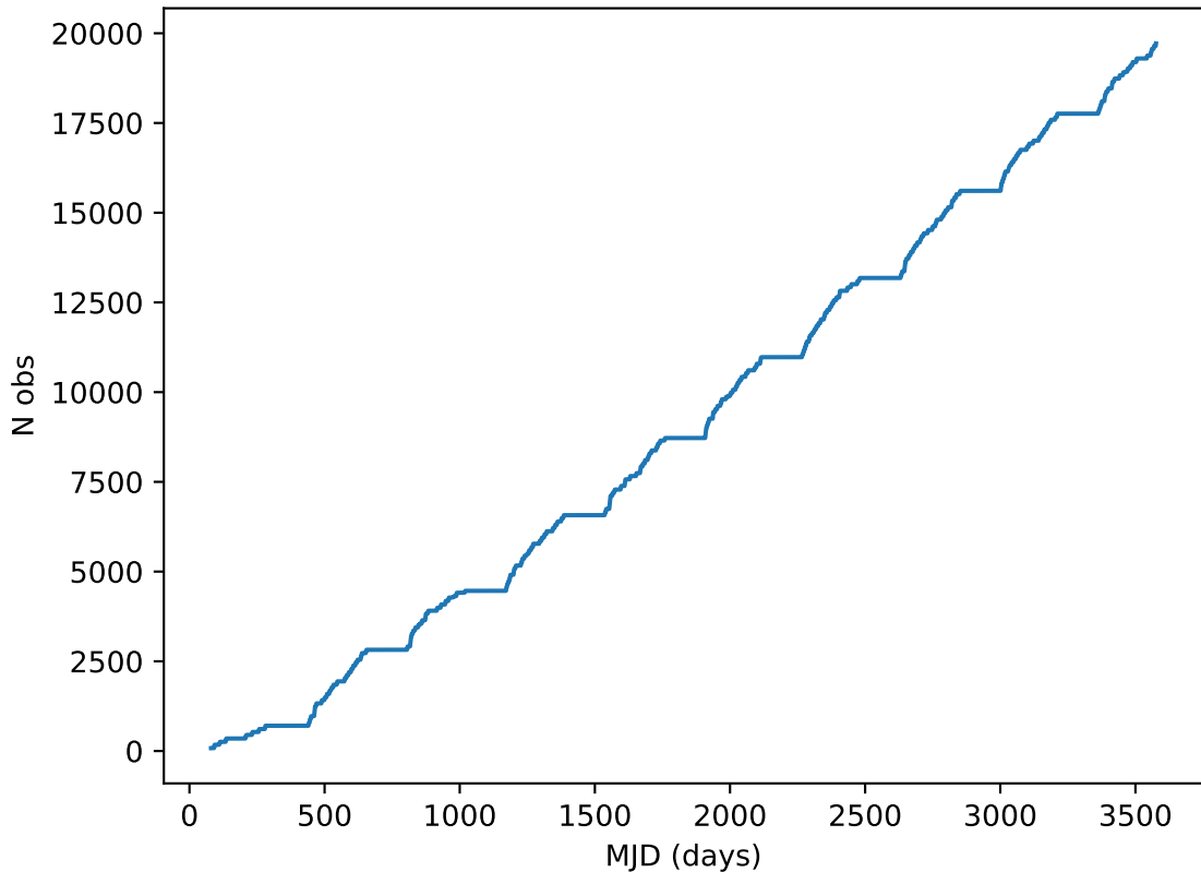
weather_cloudso20v3.4_10yrs all bands: DD:XMM_LSS Cumulative NVisits
