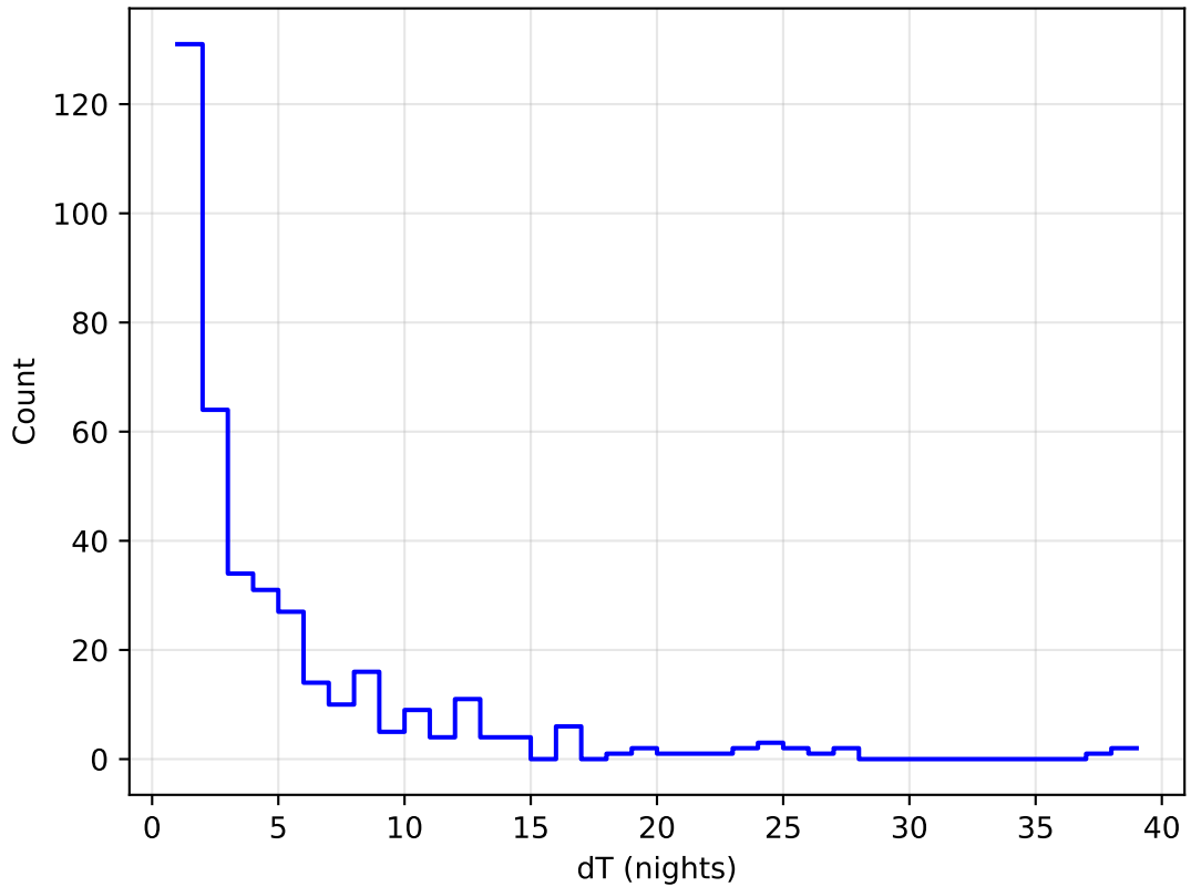
weather_cloudso20v3.4_10yrs all bands: DD:WFD Delta Nights Histogram
