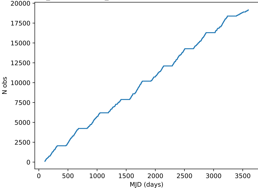
weather_cloudso20v3.4_10yrs all bands: DD:EDFS Cumulative NVisits
