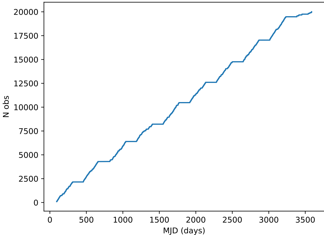
weather_cloudso20v3.4_10yrs all bands: DD:ECDFS Cumulative NVisits
