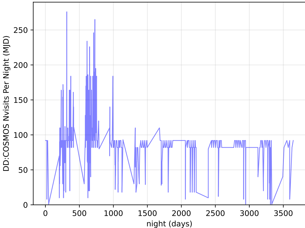
weather_cloudso20v3.4_10yrs all bands: DD: COSMOS Nvisits Per Night
