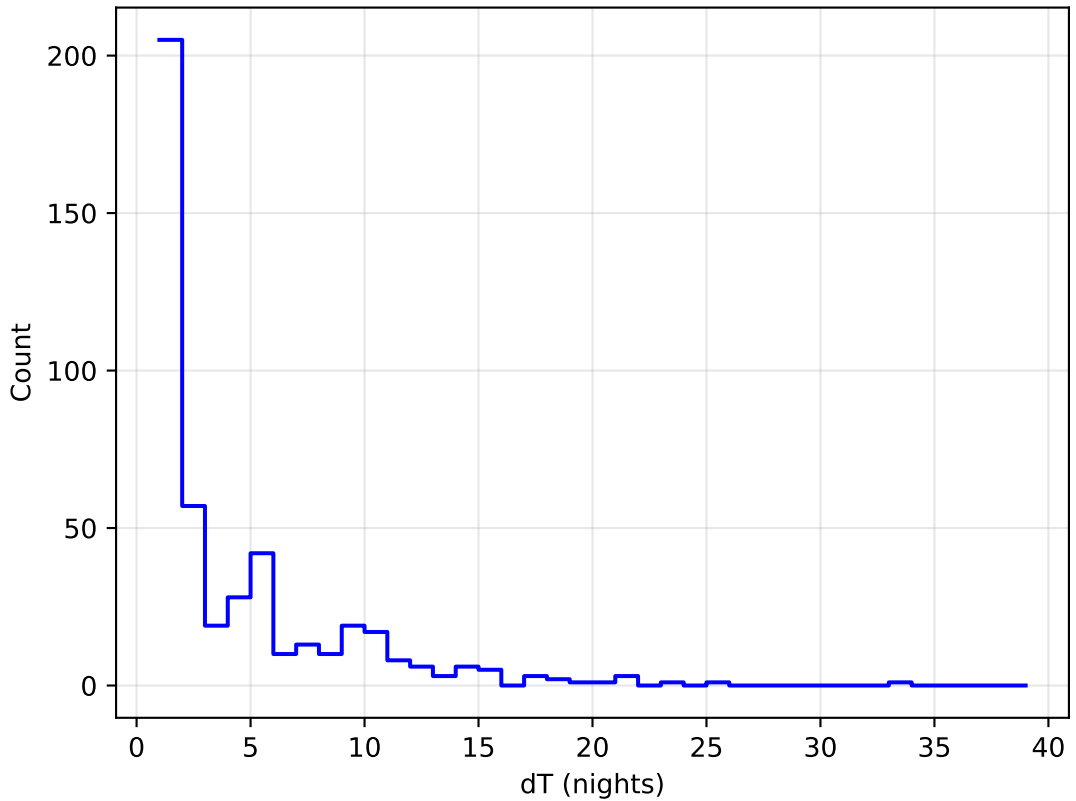
weather_cloudso20v3.4_10yrs all bands: DD: COSMOS Delta Nights Histogram
