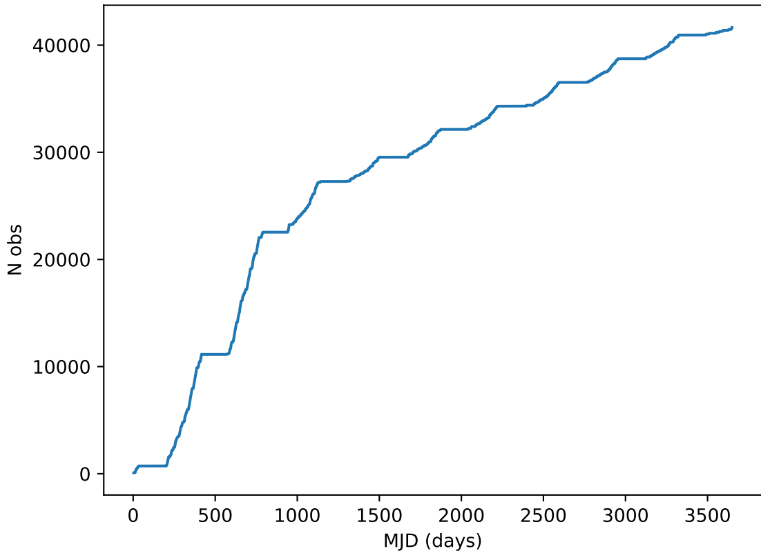
weather_cloudso20v3.4_10yrs all bands: DD:COSMOS Cumulative NVisits
