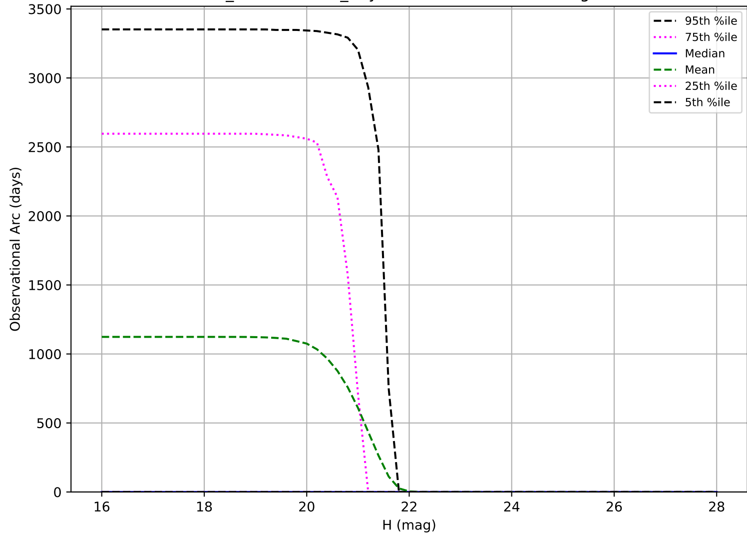
weather_cloudso1v3.4_10yrs: Observational Arc Length Vatira
