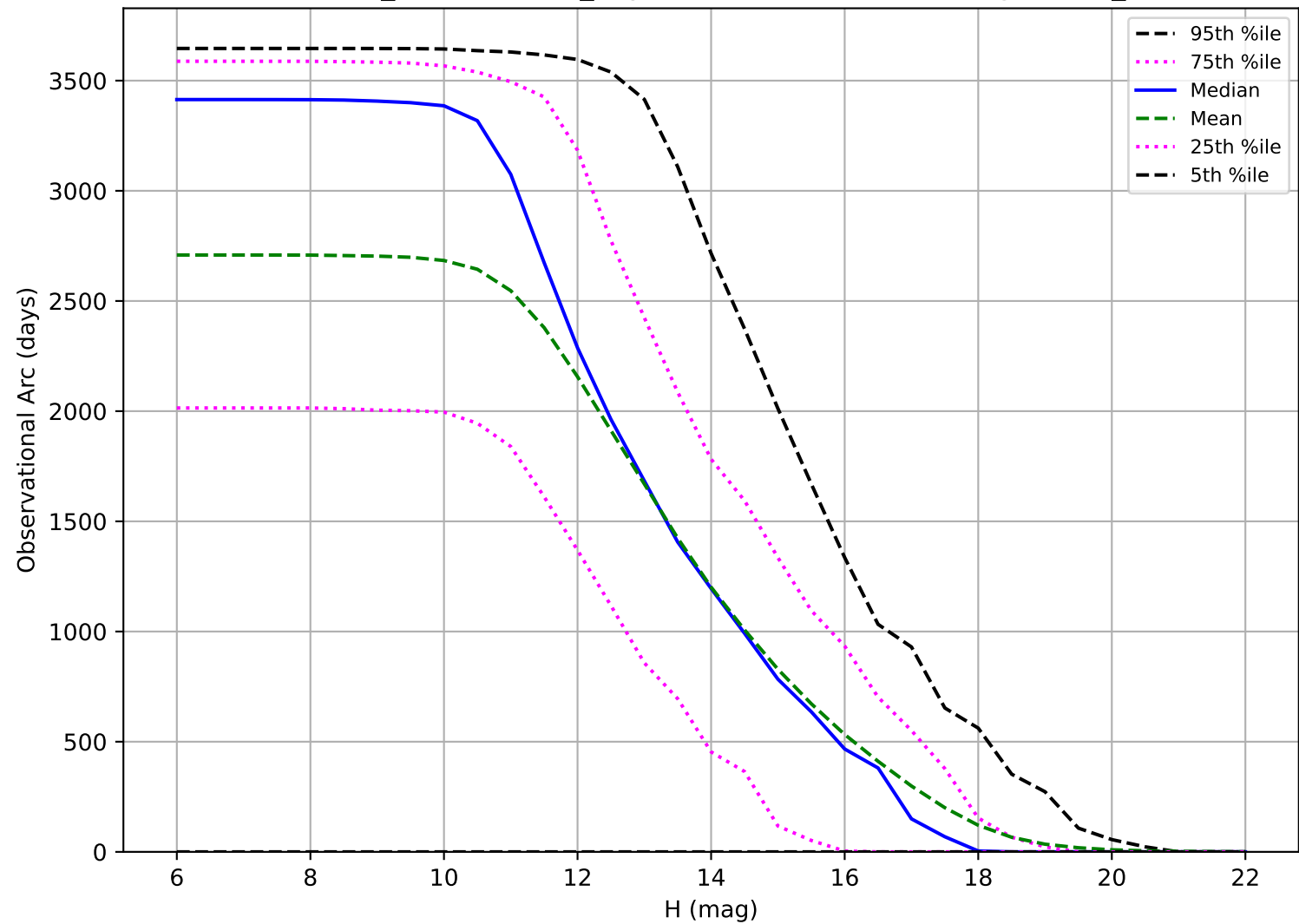
weather_cloudso1v3.4_10yrs: Observational Arc Length OCC_r5
