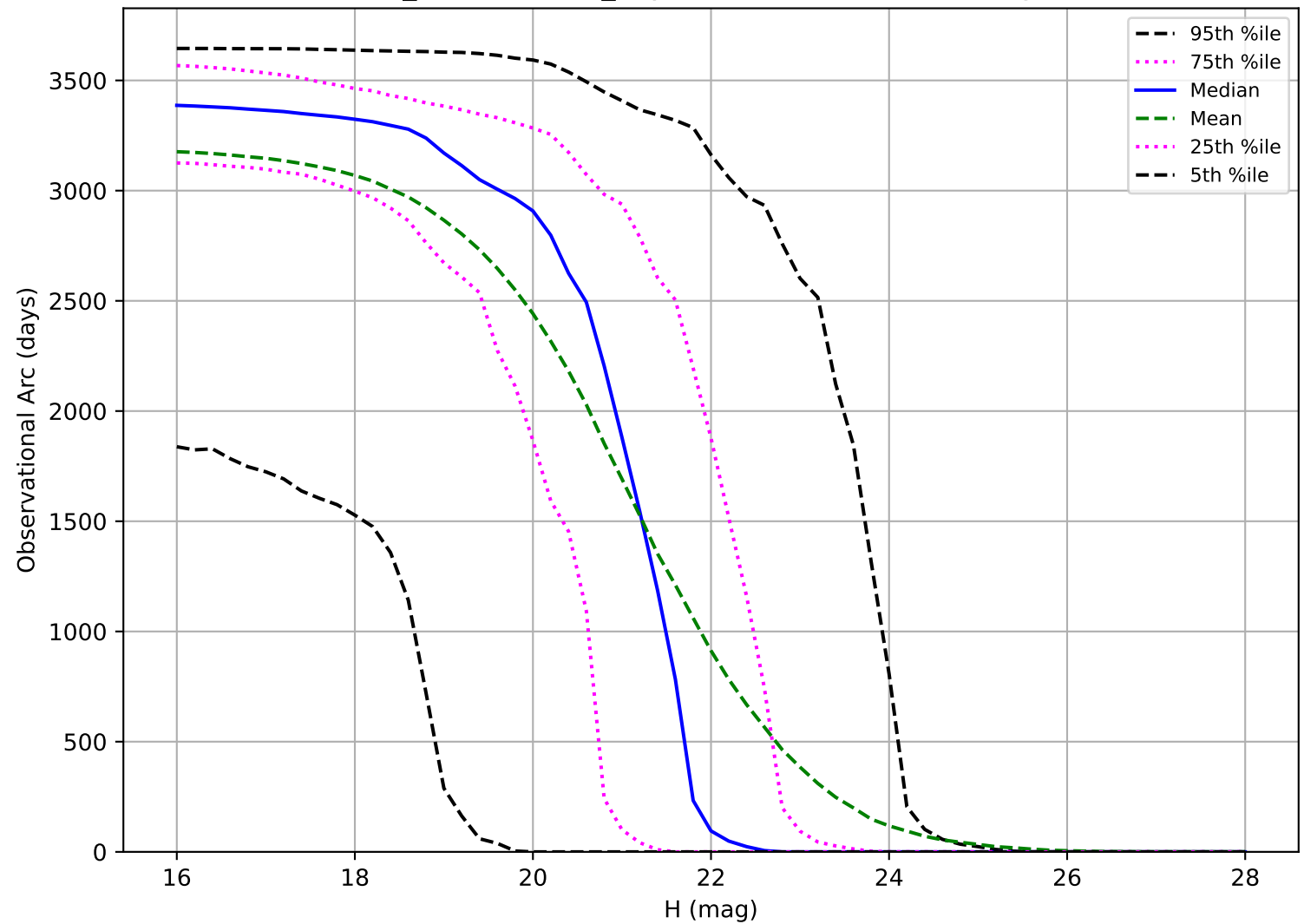
weather_cloudso1v3.4_10yrs: Observational Arc Length NEO
