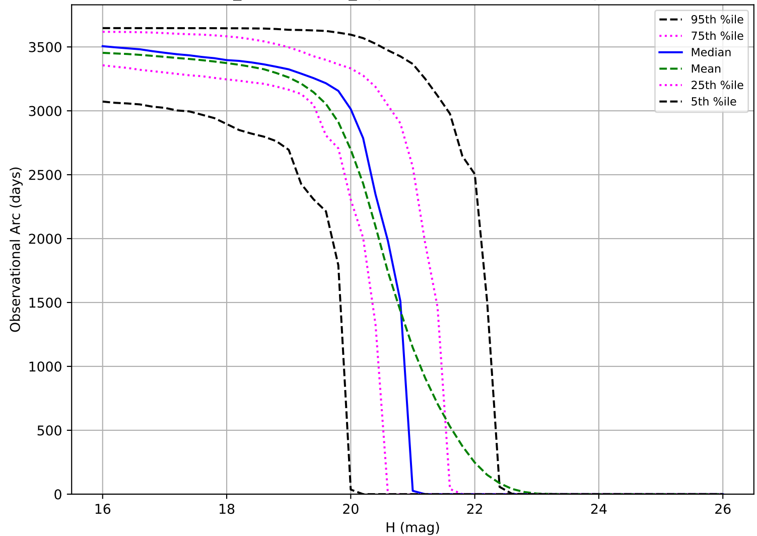
weather_cloudso1v3.4_10yrs: Observational Arc Length MBA
