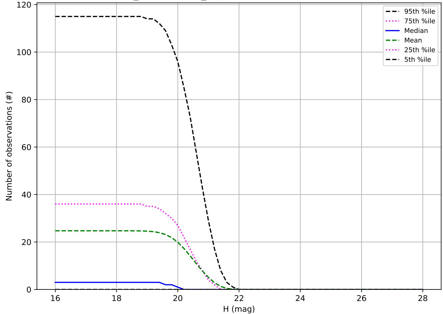
weather_cloudso1v3.4_10yrs: Number of observations Vatira
