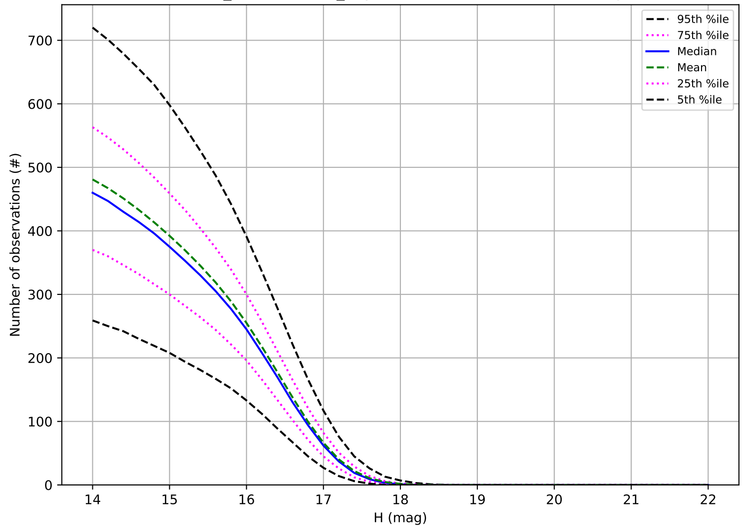
weather_cloudso1v3.4_10yrs: Number of observations Trojan
