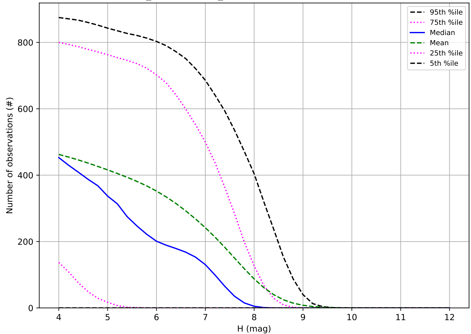
weather_cloudso1v3.4_10yrs: Number of observations TNO
