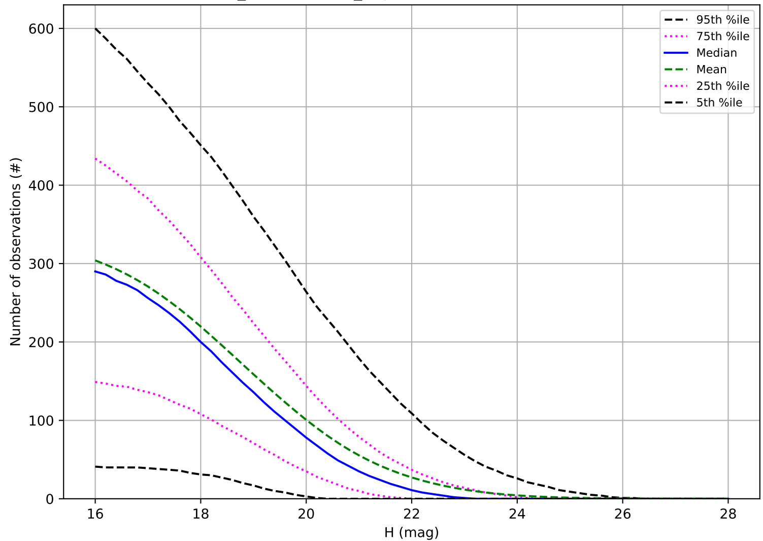
weather_cloudso1v3.4_10yrs: Number of observations PHA
